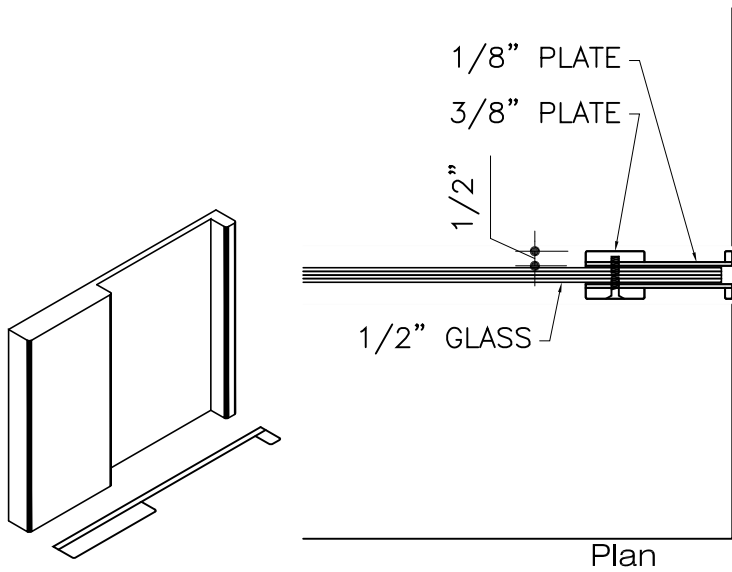
- Handle at Glass Door
