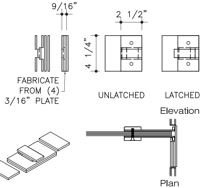
- Latch at Glass Door
